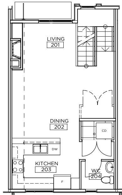
SECOND FLOOR SCALE: 1/8" = 1'-0" TYPE B - WEST
