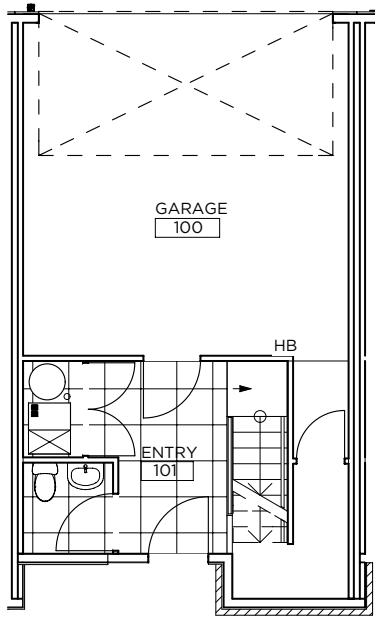
FIRST FLOOR SCALE: 1/8" = 1'-0" TYPE B - EAST
