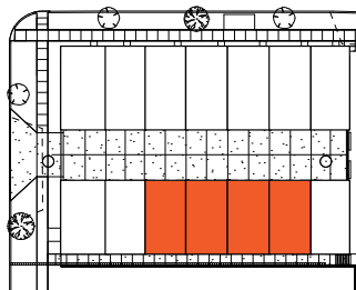
FIRST FLOOR SCALE: 1/8" = 1'-0" TYPE B - EAST
