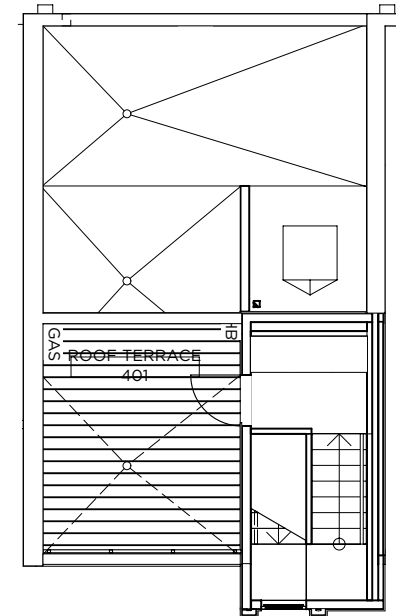
ROOFTOP SCALE: 1/8" = 1'-0" TYPE B - EAST
