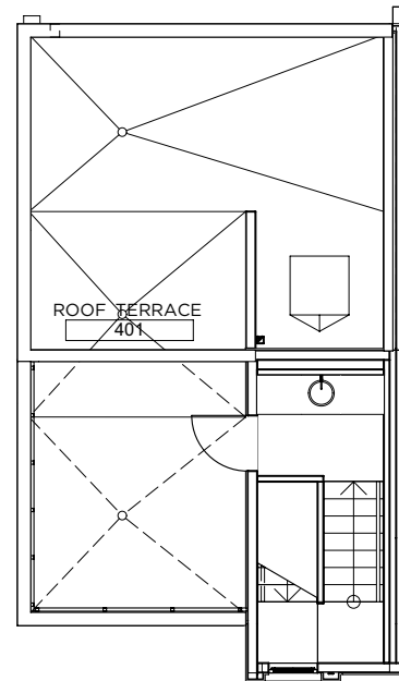
THIRD FLOOR SCALE: 1/8" = 1'-0" TYPE A - EAST
