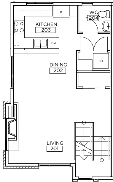
SECOND FLOOR SCALE: 1/8" = 1'-0" TYPE A - EAST
