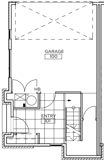
FIRST FLOOR SCALE: 1/8" = 1'-0" TYPE A - EAST
